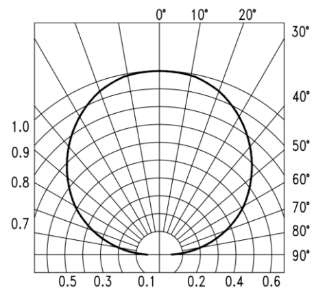
Fig.5 Radiation Characteristic Horizontal
